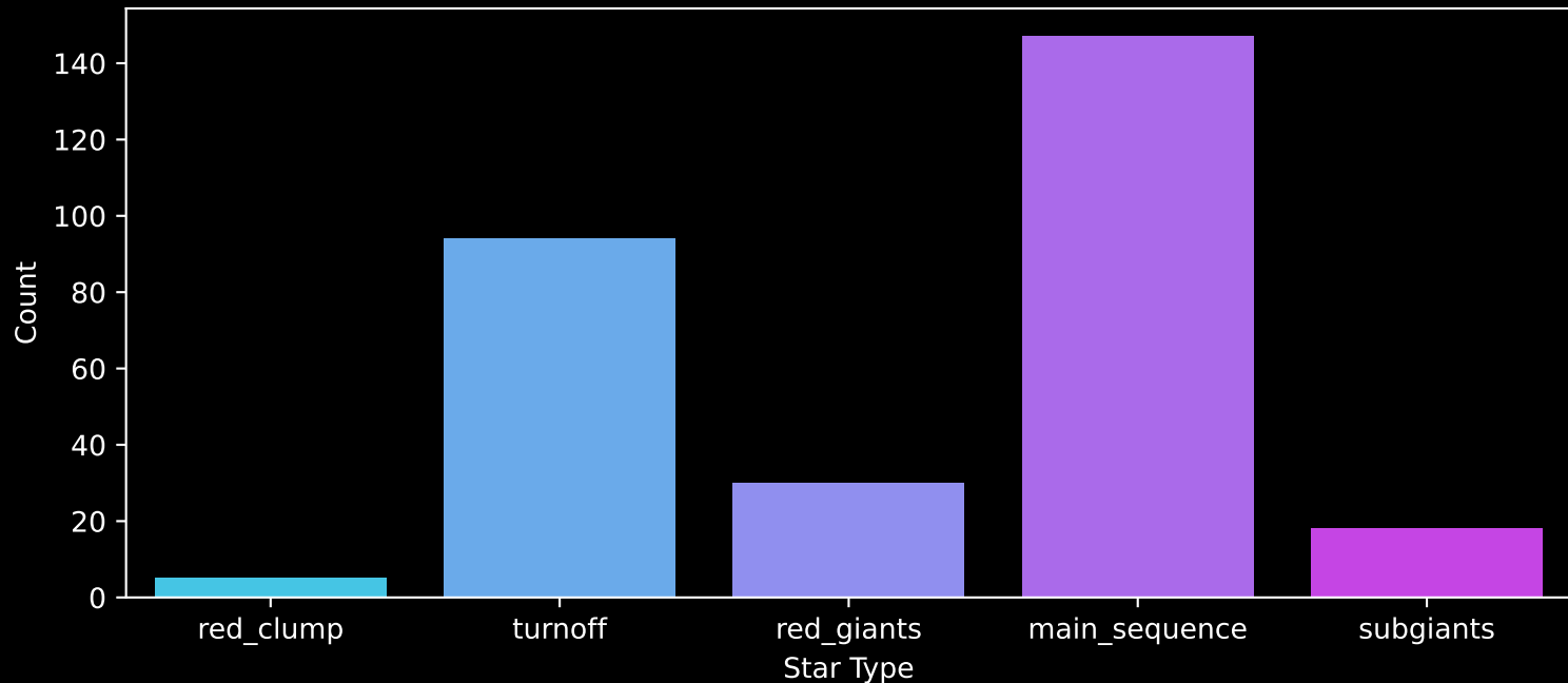
GALAH DR4 Field: [180] Count plot of Star Type
