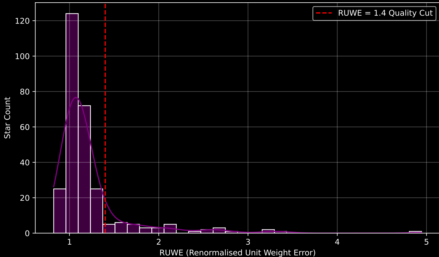
GALAH DR4 Field [180] RUWE Distribution (n= 284)
