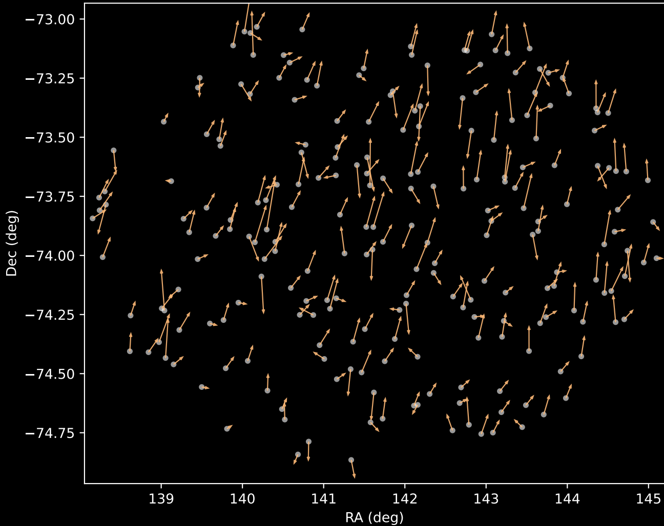
GALAH DR4 Cluster 3 Proper Motion Vectors (n=226)
